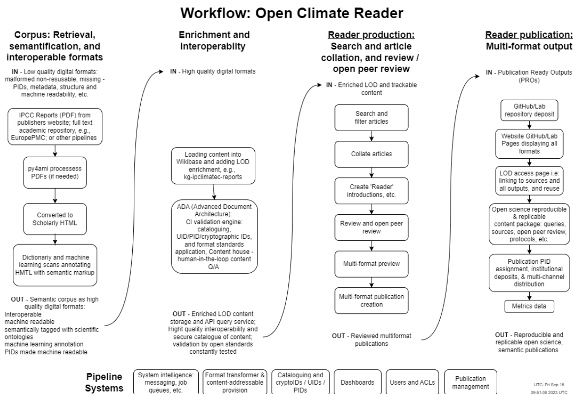
Figure 7.1: Workflow: City - Open Climate Reader
