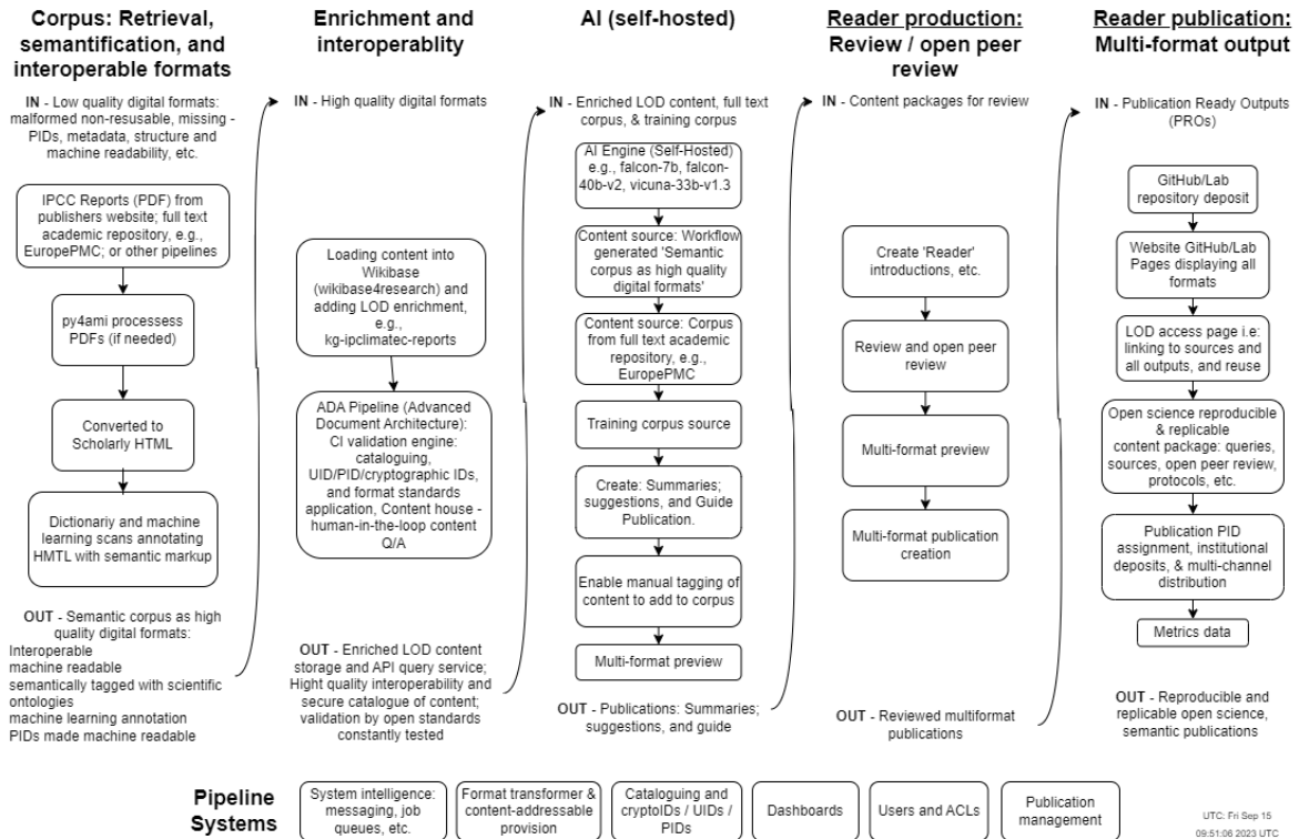
Figure 7.2: Workflow: AI Open Climate Reader
